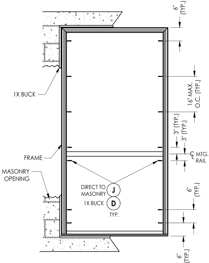
FRAME ANCHORING 1X Buck Direct to masonry
