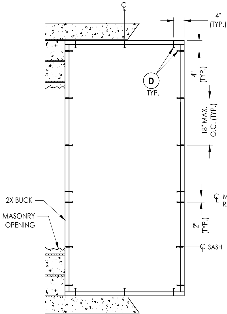
BUCK ANCHORING
